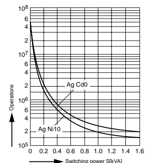
Mechanical life
